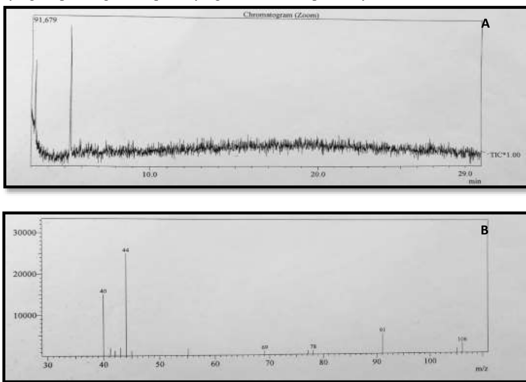
Fig. 4 (A) GCMS analysis gave two peaks of the partially purified spot at 3.23 and 5.30 minutes (B) Spectrum of the partially purified spot
